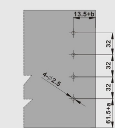
Front fixing brackets positions
