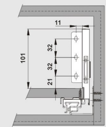
Back panel mounting positions
