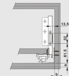
Front panel mounting positions
