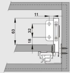
Back panel mounting positions
