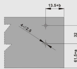
Front fixing brackets positions
