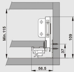
Inside cabinet dimension
