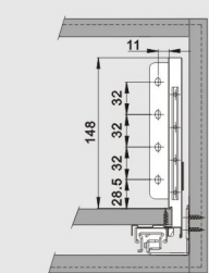
Back panel mounting positions
