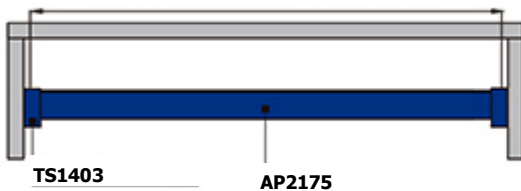
Inner cabinet width less 12mm
