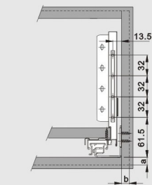
Front panel mounting positions
