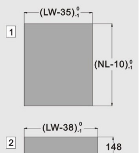
H120mm back and base
