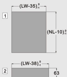
H80mm back and base
