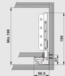
Inside cabinet dimension
