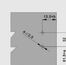
Front fixing brackets positions
