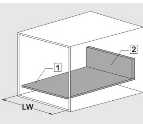
H80mm back and base
