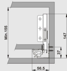
Inside cabinet dimension
